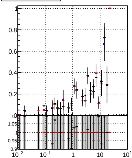
Fake rate vs v Legend: —•— /data2/legianni/JSON-bkwd-fwd/no-modif/CMSSW_13_0_X_2023-01-24-1100/src/DQM_original —•— DQM_modified —•— DQM_modified_4iter-NewERR
