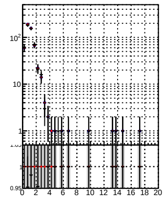
N of reco track vs. \chi^2 - blue: /data2/legion/JSON-bkwd-fwd/no-modif/CMSSW_13_0_X_2023-01-24-1100/src/DQM_original - red: DQM modified - black: DQM modified 4iter-NewERR
