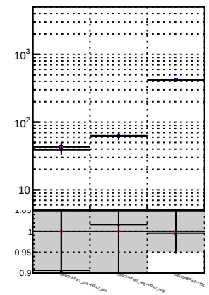
N of reco track vs. \chi^2 - blue: /data2/legion/JSON-bkwd-fwd/no-modif/CMSSW_13_0_X_2023-01-24-1100/src/DQM_original - red: DQM modified - black: DQM modified 4iter-NewERR
