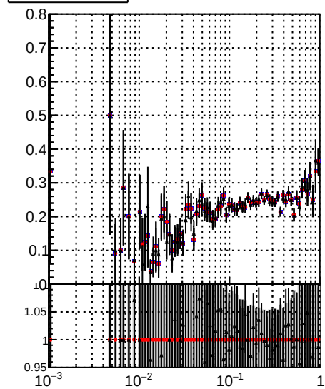
/data2/legianni/JSON-bkwd-fwd/no-modif/CMSSW_13_0_X_2023-01-24-1100/src/DQM_original Fake rate vs DQM_modified DQM_modified_4iter-NewERR
