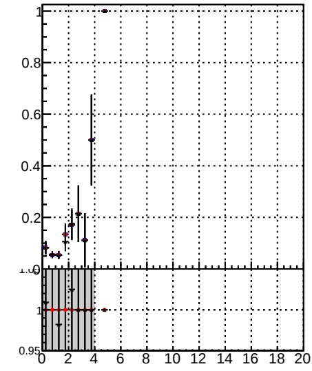
Fake rate vs. \chi^2 for BQM modified 4iter-NewERR
