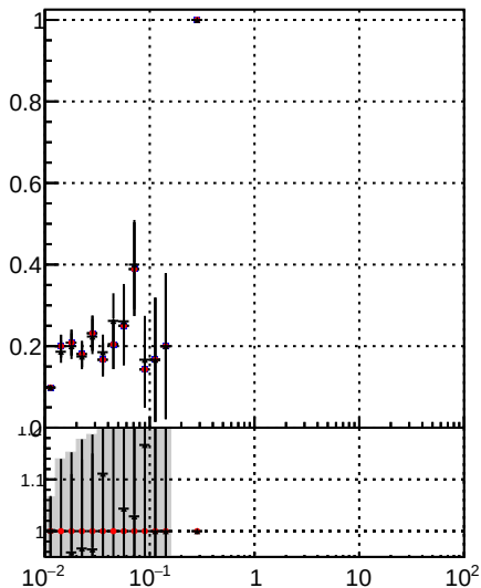
Legend: /data2/legianni/JSON-bkwd-fwd/no-modif/CMSSW_13_0_X_2023-01-24-1100/src/DQM_original (black), DQM_modified (red), DQM_modified_4iter-NewERR (grey)
