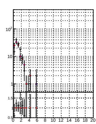
Legend: - \chi^2 modified 4iter-NewERR - \chi^2 modified - \chi^2 original - \chi^2 bkwd-fwd/no-modif - \chi^2 bkwd-fwd/no-modif/CMSSW_13_0_X_2023-01-24-1100/src/DQM_original
