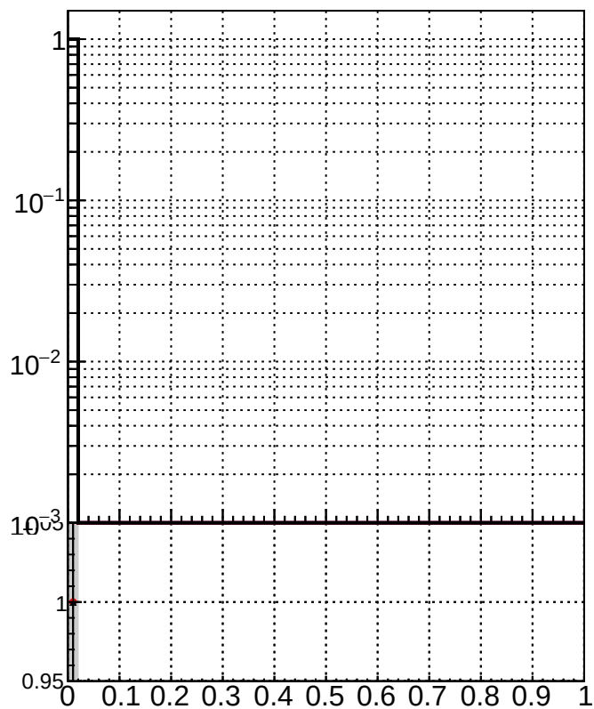
RecoPVAssoc2GenPVNotMatched_Purity
