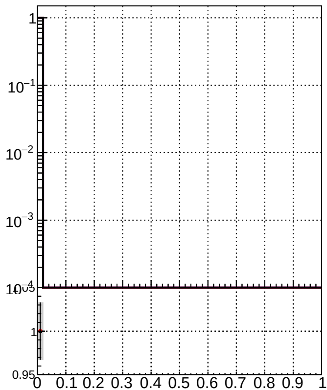
RecoPVAssoc2GenPVMatched_Purity
