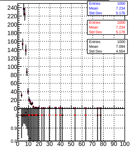
Uncertainty z Coordinate (tagged Vtx)
