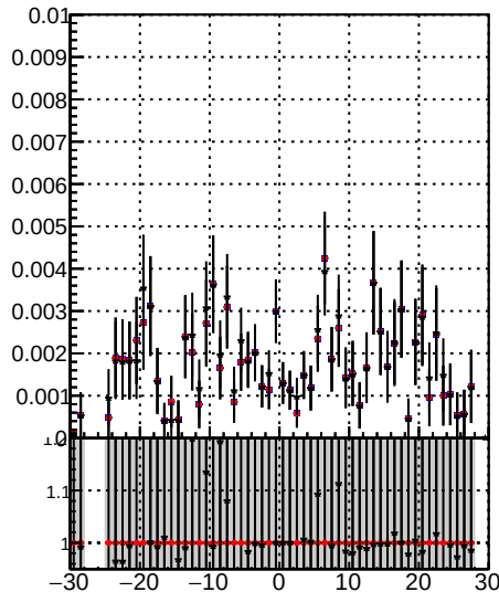
Fake rate vs d —•— /data2/legianni/JSON-bkwd-fwd/no-modif/CMSSW_13_0_X_2023-01-24-1100/src/DQM_original —•— BQM modified 4iter-NewERR
