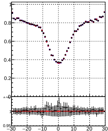
Fake rate vs d —•— /data2/legianni/JSON-bkwd-fwd/no-modif/CMSSW_13_0_X_2023-01-24-1100/src/DQM_original —•— BQM modified 4iter-NewERR
