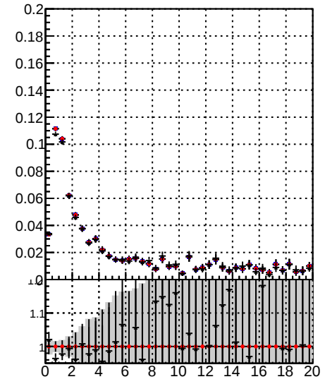
Fake rate vs. /data2/legianni/JSON-bkwd-fwd/no-modif/CMSSW_13_6_X_2023-01-24-1100/src/DQM_original DQM modified 4iter-NewERR
