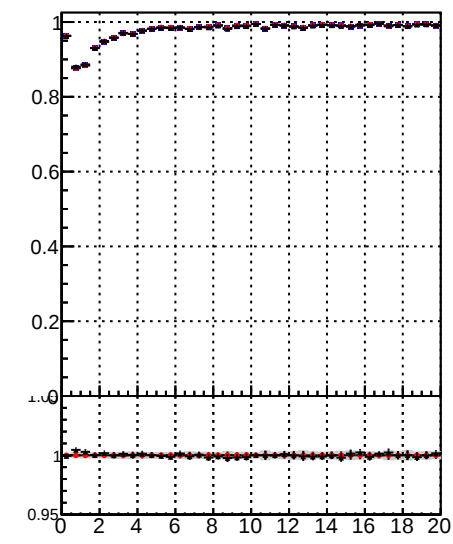
Fake rate vs. /data2/legianni/JSON-bkwd-fwd/no-modif/CMSSW_13_6_X_2023-01-24-1100/src/DQM_original DQM modified 4iter-NewERR
