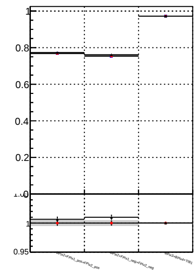
Fake rate vs. /data2/legianni/JSON-bkwd-fwd/no-modif/CMSSW_13_6_X_2023-01-24-1100/src/DQM_original DQM modified 4iter-NewERR
