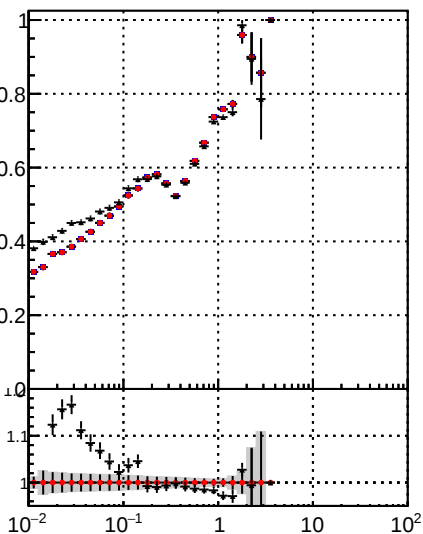
/data2/legianni/JSON-bkwd-fwd/no-modif/CMSSW_13_0_X_2023-01-24-1100/src/DQM_original Fake rate vs vertpos DQM_modified DQM_modified_4iter-NewERR
