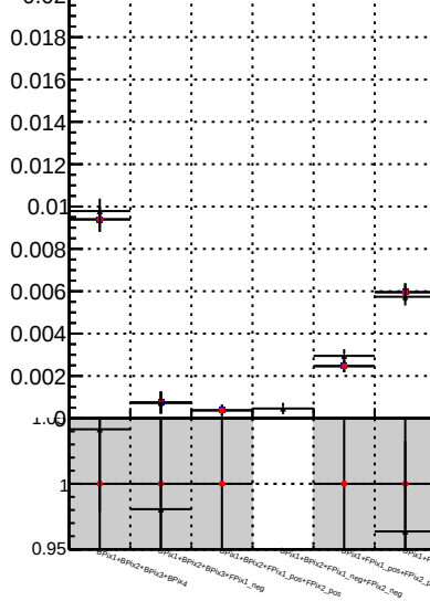
Duplicates Rate vs.
