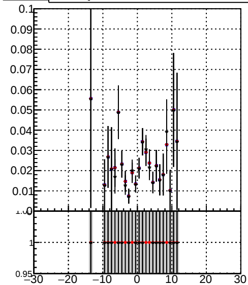
Efficiency Legend: /data2/legianni/JSON-bkwd-fwd/no-modif/CMSSW_13_0_X_2023-01-24-1100/src/DQM_original DQM_modified DQM_modified_4iter-NewERR
