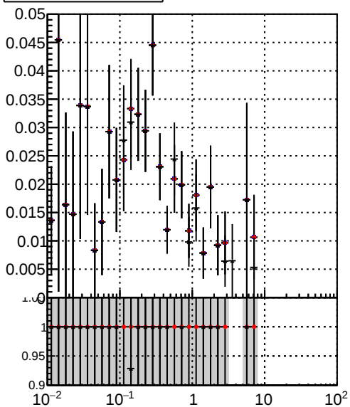
Efficiency Legend: /data2/legianni/JSON-bkwd-fwd/no-modif/CMSSW_13_0_X_2023-01-24-1100/src/DQM_original DQM_modified DQM_modified_4iter-NewERR
