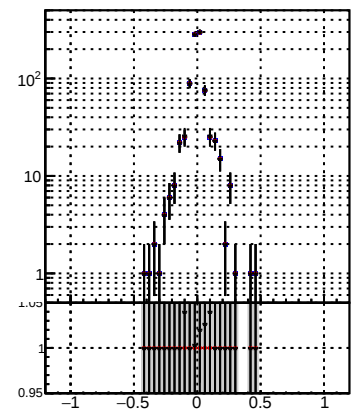
N of associated tracks (simToReco) vs dz(PV) zoomed in
