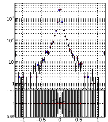
N of simulated tracks vs dz(PV) zoomed
