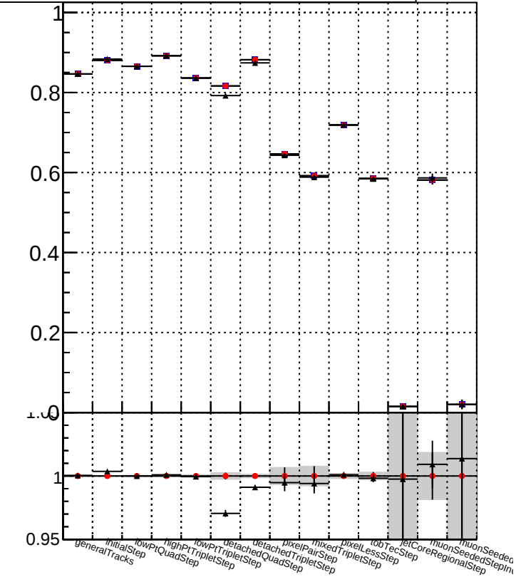
Duplicates rate vs collection Legend: /data2/legianni/JSON-bkwd-fwd/no-modif/CMSW_13_0_X_2023-01-24-1100/src/DQM_original DQM_modified DQM_modified_4iter-NewERR
