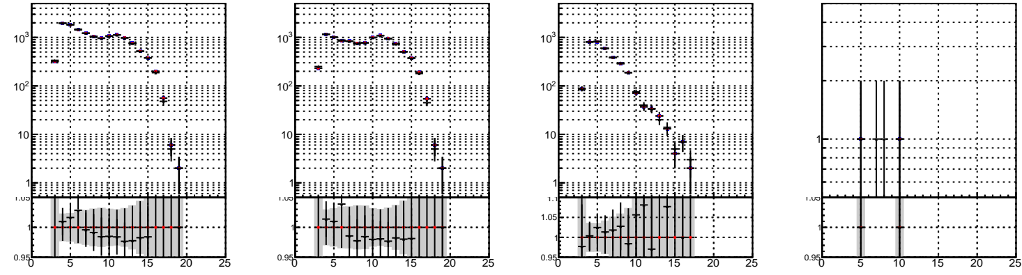
Legend: - Blue line with dots: /data2/legianni/JSON-bkwd-fwd/no-modif/CMSSW_13_0_X_2023-01-24-1100/src/DQM_original - Red line with dots: DQM modified - Black line with dots: 4iter-NewERR - Grey shaded area: 4iter-NewERR - Black histogram: 4iter-NewERR - Red horizontal line: 4iter-NewERR - Grey shaded area: 4iter-NewERR - Black histogram: 4iter-NewERR - Red horizontal line: 4iter-NewERR
