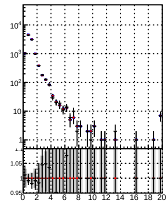
N of reco track vs. \chi^2 for data2/legion1/JSON-bkwd-fwd/no-modif/CMSSW_13_0_X_2023-01-24-1100/src/DQM_modified 4iter-NewERR
