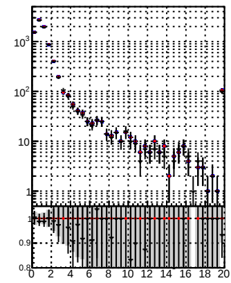
N of reco track vs. \chi^2 for /data2/legion/jason-bkwd-fwd/no-modif/CMSSW_13_0_X_2023-01-24-1100/src/DQM_original (blue dots), /data2/legion/jason-bkwd-fwd/no-modif/CMSSW_13_0_X_2023-01-24-1100/src/DQM_modified (black dots), and /data2/legion/jason-bkwd-fwd/no-modif/CMSSW_13_0_X_2023-01-24-1100/src/DQM_modified_4iter-NewERR (red dots).
