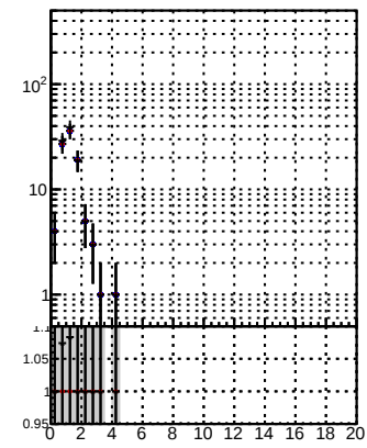
N of reco track vs. \chi^2 for \sqrt{s}=13 TeV, 36.1 fb ^{-1} data, 4iter-NewERR
