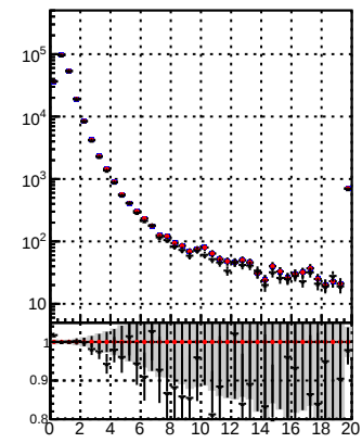
N of reco track vs. \chi^2 data2/legsim/JSON-bkwd-fwd/no-modif/CM3SW_13_0_X_2023-01-24-1100/src/DQM_original DOM modified 4iter-NewERR
