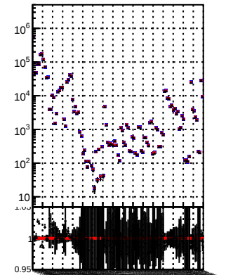
N of reco track vs. \chi^2 data2/legsim/JSON-bkwd-fwd/no-modif/CMSSW_13_0_X_2023-01-24-1100/src/DQM_original DQM modified 4iter-NewERR
