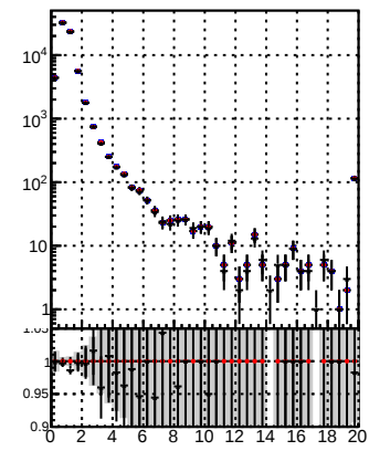
N of reco track vs. \chi^2 data2/legsim/JSON-bkwd-fwd/no-modif/CMSSW_13_0_X_2023-01-24-1100/src/DQM_original
