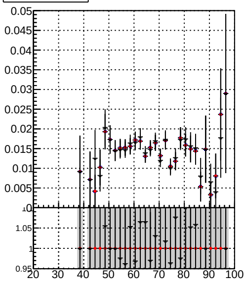
Efficiency vs \Delta R(\text{track}, \text{jet})
