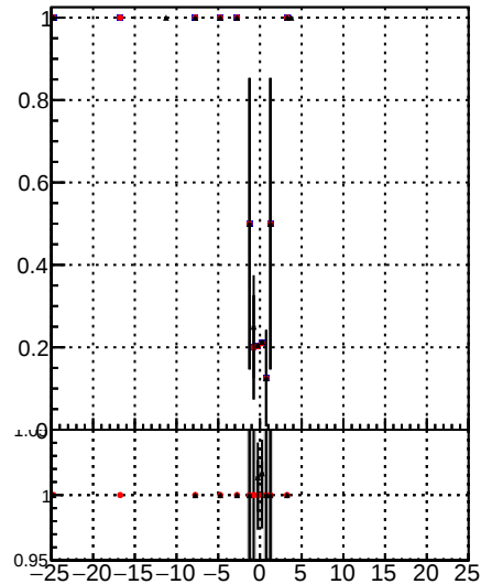
Fake rate vs d /data2/legianni/JSON-bkwd-fwd/no-modif/CMSSW_13_0_X_2023-01-24-1100/src/DQM_original DQM modified 4iter-NewERR
