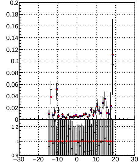
/data2/legianni/JSON-bkwd-fwd/no-modif/CMSSW_13_0_X_2023-01-24-1100/src/DQM_original BQM_modified_4iter-NewERR
