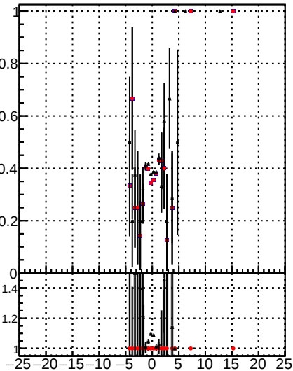
/data2/legianni/JSON-bkwd-fwd/no-modif/CMSSW_13_0_X_2023-01-24-1100/src/DQM_original BQM_modified_4iter-NewERR
