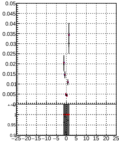
/data2/legianni/JSON-bkwd-fwd/no-modif/CMSSW_13_0_X_2023-01-24-1100/src/DQM_original BQM_modified_4iter-NewERR
