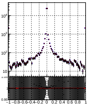
N of sim DQM_modified_4iter-N
