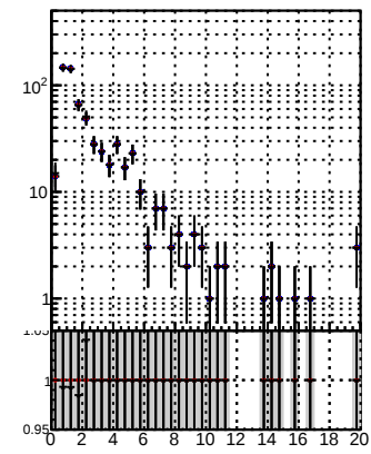
N of reco track vs. \chi^2 for different categories: - data2legion/JSON-bkwd-fwd/no-modif/CMSSW_13_0_X_2023-01-24-1100/src/DQM_original (blue) - DQM modified 4iter-NewERR (red) - DQM modified (green)
