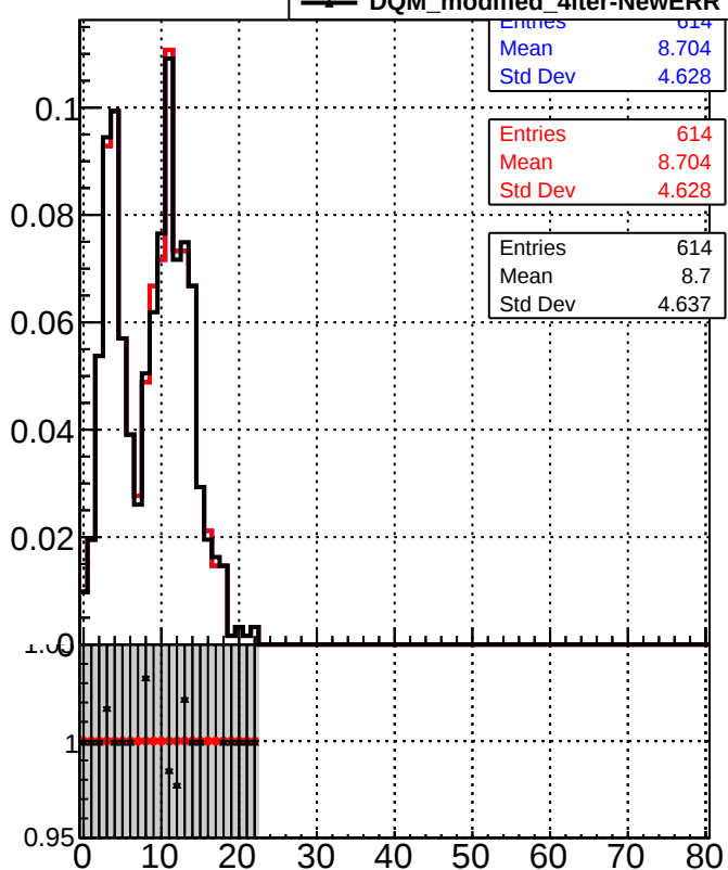
Legend for bottom row: /data2/legianni/JSON-bkwd-fwd/no-modif/CMSSW_13_0_X_2023-01-24-1100/src/DQM_original (Blue) DQM_modified (Red) DQM_modified_4iter-NewERR (Black)
