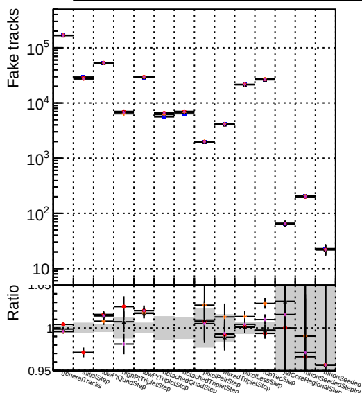
Number Symbol Model Fit Test Update Error 1 Black triangle DOM mkFit TT JanUpdate statErr 2 Orange square DOM mkFit TT JanUpdate systErr 3 Purple circle DOM mkFit TT JanUpdate bothErr
