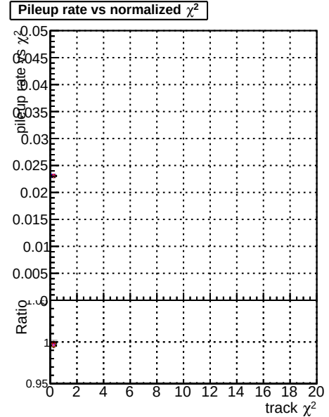
Pileup rate vs normalized \chi^2
