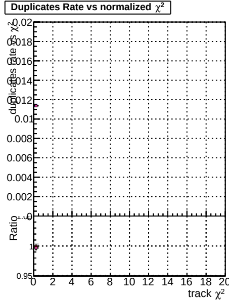
Duplicates Rate vs normalized \chi^2
