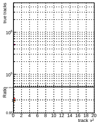
N of associated (recoToSim) tracks vs. \chi^2 for different \chi^2 bins
