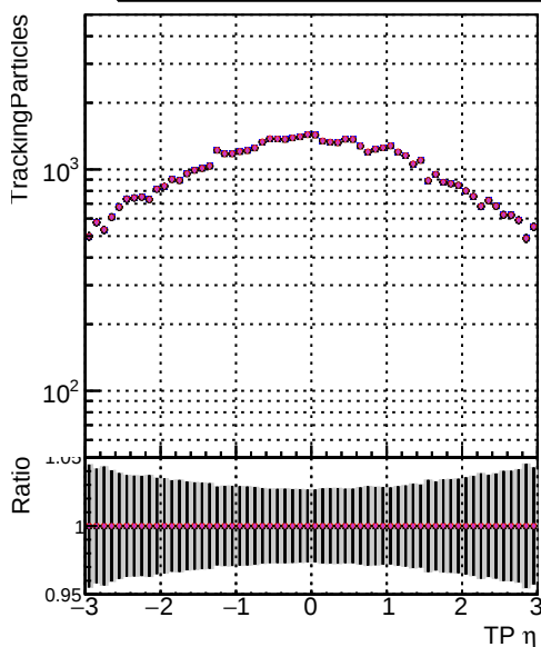
N of sim Model Method Time Update Stat Err 100 DOM mkFit TT Jan Update statErr 100 DOM mkFit TT Jan Update systErr 100 DOM mkFit TT Jan Update bothErr
