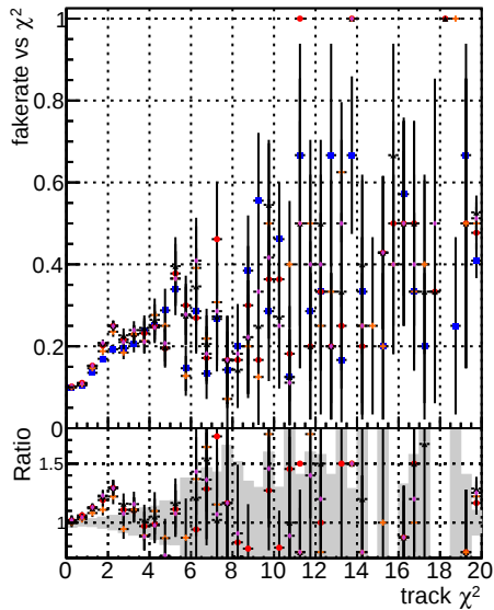
Fake rate vs. DOM mkFit DOM mkFit T DOM mkFit T original
