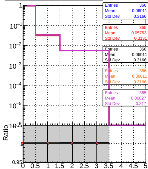
Legend: DOM mkFit TT original, DOM mkFit TT JanUpdate-noErr, DOM mkFit TT JanUpdate-statErr, DOM mkFit TT JanUpdate-systErr, DOM mkFit TT JanUpdate-bothErr mean hit
