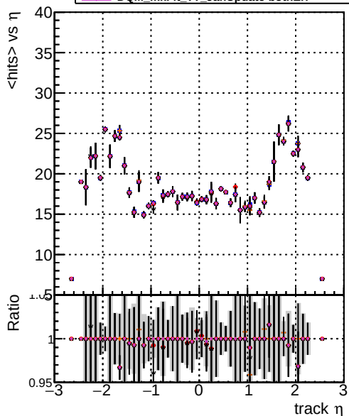
Legend: DOM mkFit TT original, DOM mkFit TT JanUpdate-noErr, DOM mkFit TT JanUpdate-statErr, DOM mkFit TT JanUpdate-systErr, DOM mkFit TT JanUpdate-bothErr mean hit
