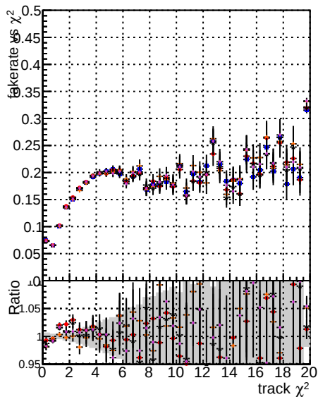
Fake rate vs. DOM mkrfit T original DOM mkrfit T Jan Update 2015 DOM mkrfit T Jan Update 2016
