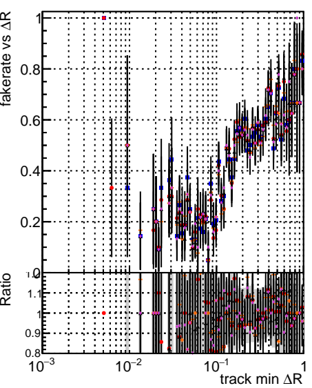
Fake rate vs \Delta R(\text{track, jet}) DOM mkFit TronFit Original JanUpdata noEr BSMER
