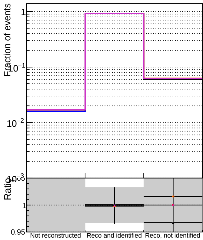
TruePVLocationIndexInRecoVertexCollectionCumulative
