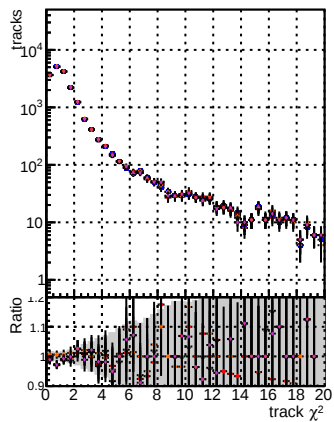
N of reco track vs. \chi^2 for B0M, mFit, and Original tracks
