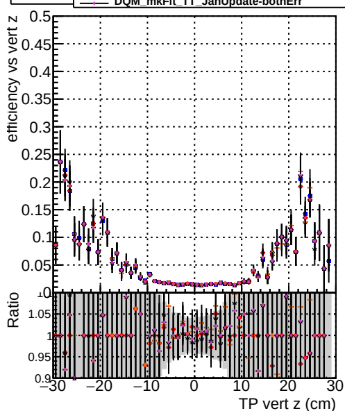
Efficiency Model Method Dataset Update Error 0.95 DOM mkFit TT JanUpdate statErr 0.90 DOM mkFit TT JanUpdate systErr 0.85 DOM mkFit TT JanUpdate bothErr
