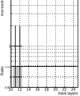
N of associated (recoToSim) tracks vs layer
