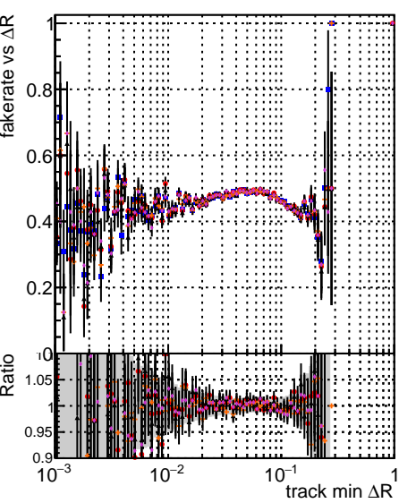
Fake rate vs DOM mkFit T-Original JanUpdata noEr DOM mkFit T-Original JanUpdata noEr DOM mkFit T-Original JanUpdata noEr DOM mkFit T-Original JanUpdata noEr DOM mkFit T-Original JanUpdata noEr DOM mkFit T-Original JanUpdata noEr DOM mkFit T-Original JanUpdata noEr DOM mkFit T-Original JanUpdata noEr DOM mkFit T-Original JanUpdata noEr DOM mkFit T-Original JanUpdata noEr
