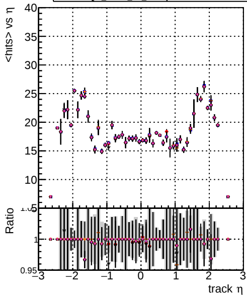
Legend: DOM mkFit (blue line) DOM mkFit (red line) DOM mkFit (orange line) DOM mkFit (purple line) JanUpdate-noErr (black line) JanUpdate-statErr (black line) JanUpdate-systErr (black line) JanUpdate-bothErr (black line)
