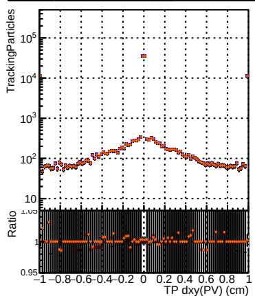
N of sim —▲— DQM_mkFit_TT_JanUp —●— DQM_mkFit_TT_JanUp
