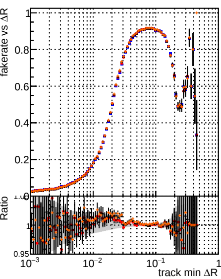
Fake rate vs \Delta R(\text{track, jet}) Legend: DOM mkFit T original DOM mkFit T JanUpdate noErr DOM mkFit T JanUpdate statErr DOM mkFit T JanUpdate systErr
