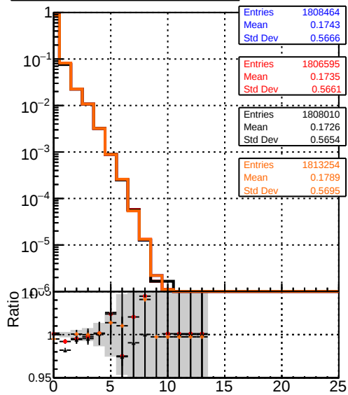
mean hit Ratio track \eta DOM_mkFit_TToriginal DOM_mkFit_TT_JanUpdate-noErr DOM_mkFit_TT_JanUpdate-statErr DOM_mkFit_TT_JanUpdate-systErr
