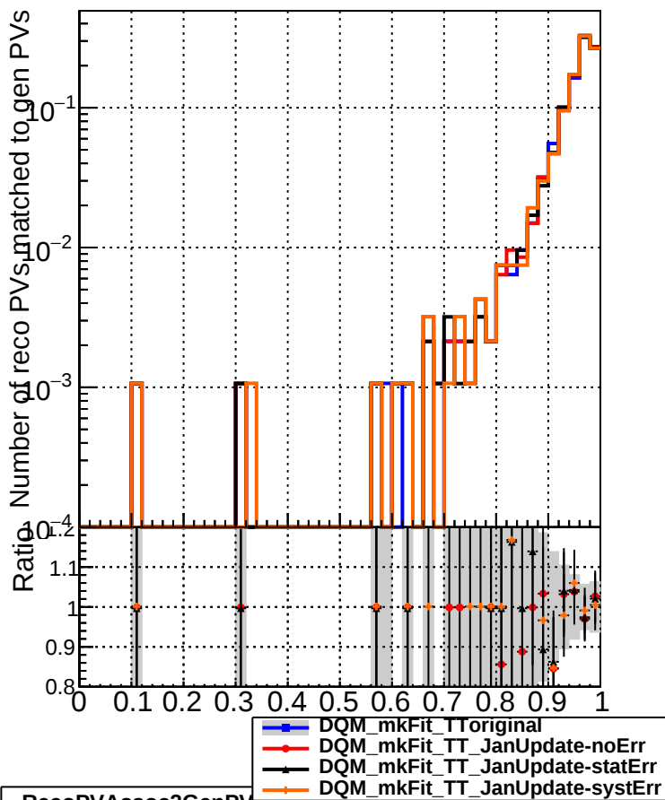
RecoPVAssoc2GenPVmatched_missing
