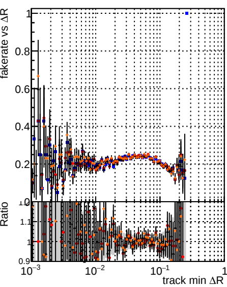
Fake rate vs \Delta R (track, jet) Legend: DOM mkFit Original DOM mkFit JanUpdate noErr DOM mkFit JanUpdate statErr DOM mkFit JanUpdate systErr
