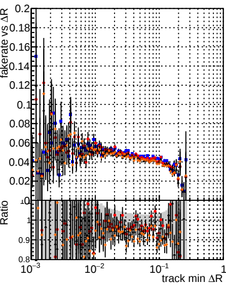
Fake rate vs \Delta R(\text{track, jet}) Legend: DOM mktFit Toriginal DOM mktFit JanUpdate-noErr DOM mktFit JanUpdate-statErr DOM mktFit JanUpdate-systErr
