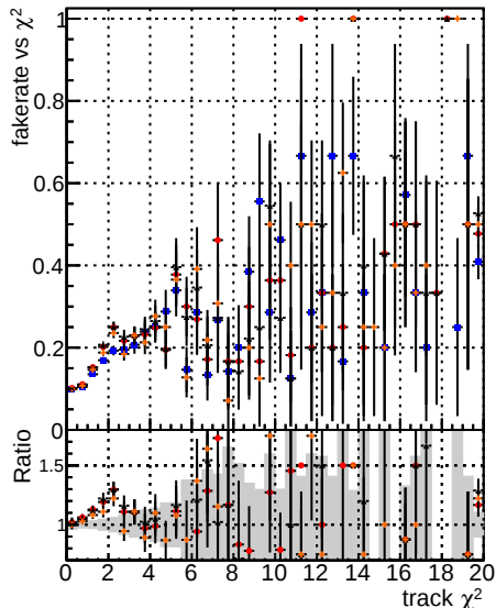
Fake rate vs. DQM mkFit Ttoriginal DQM mkFit Ttupdate system
